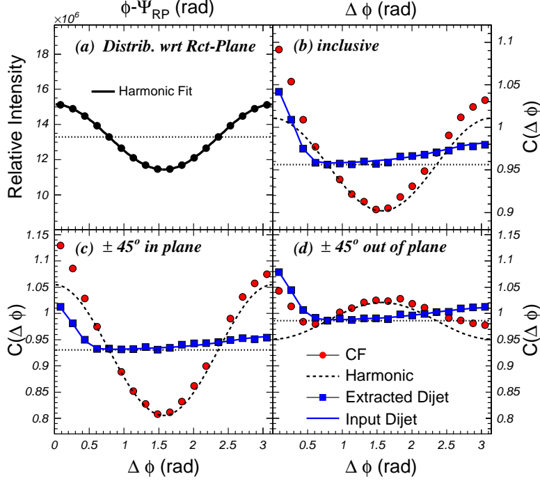
Fig. 3. Simulation test of the ZYAM decomposition procedure from [ 39]. (a) simulated azimuthal distribution of particles with respect to the event plane. (b) Simulated correlation function with harmonic component and extracted jet-pair distribution. The solid line represents the input jet-pair distribution (referenced to a_o ) as obtained from tagging the jet particles in the simulation. (c) and (d) same as (b) but for trigger particles constrained in-plane and out-of-plane respectively (see text).
